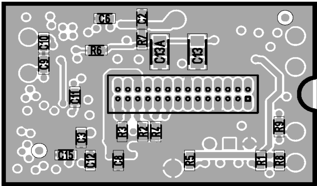
Figure 4-2. Solder Side
